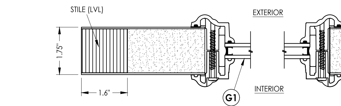
1 4 HORIZONTAL CROSS SECTION
