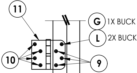
HINGE DETAIL 1
