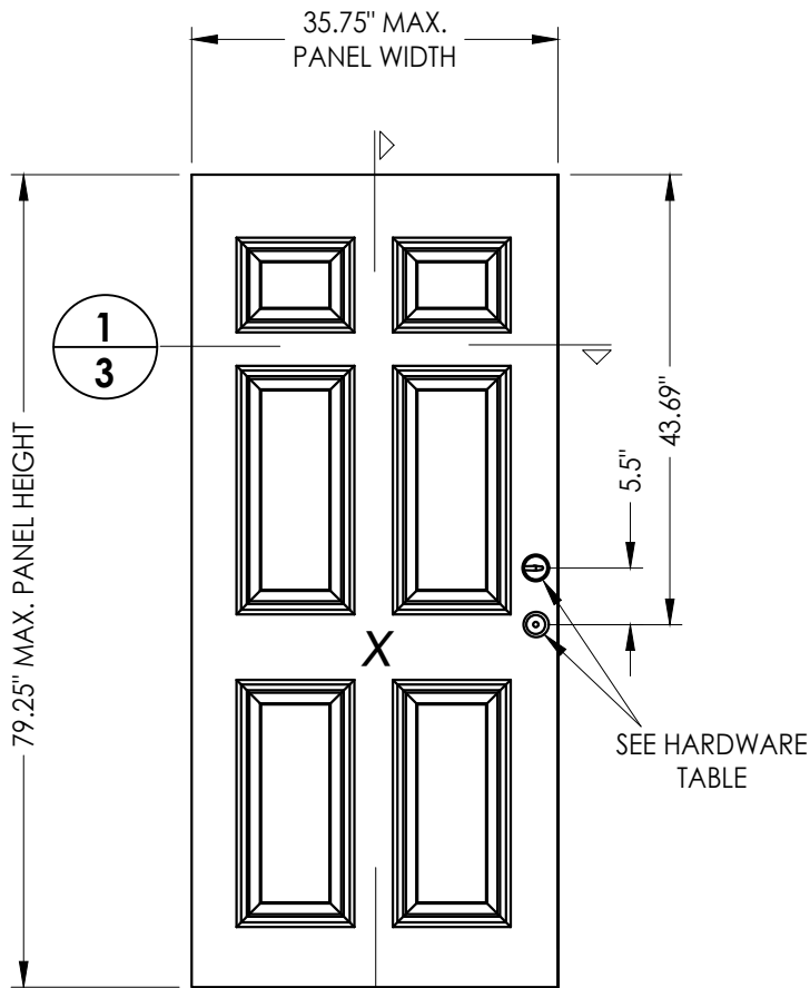
2 3 DOOR PANEL Masonite Fiberglass
