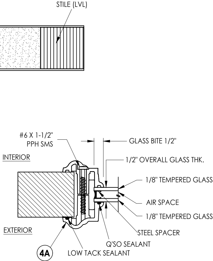
G1 GLAZING DETAIL
